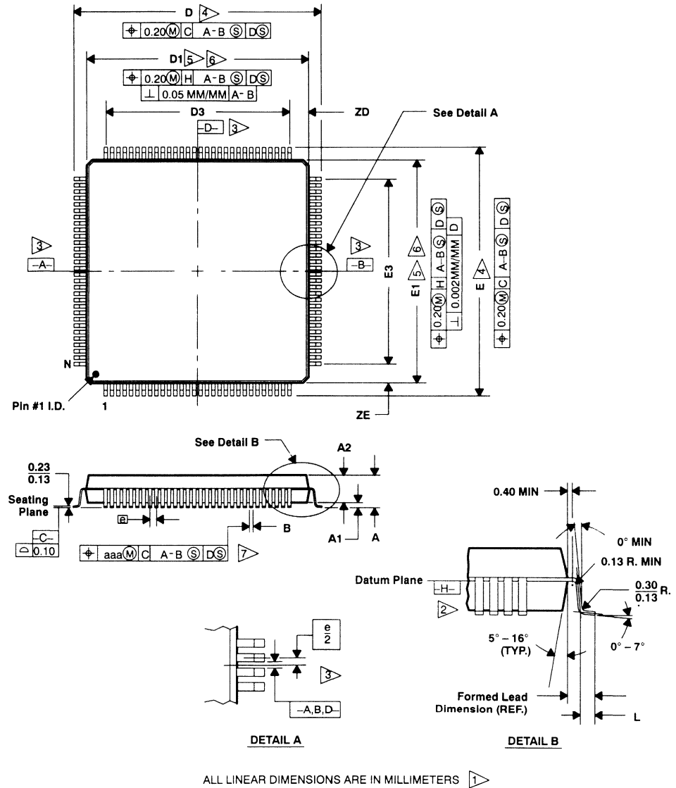
Figure 45. Plastic Quad Flat Packages
