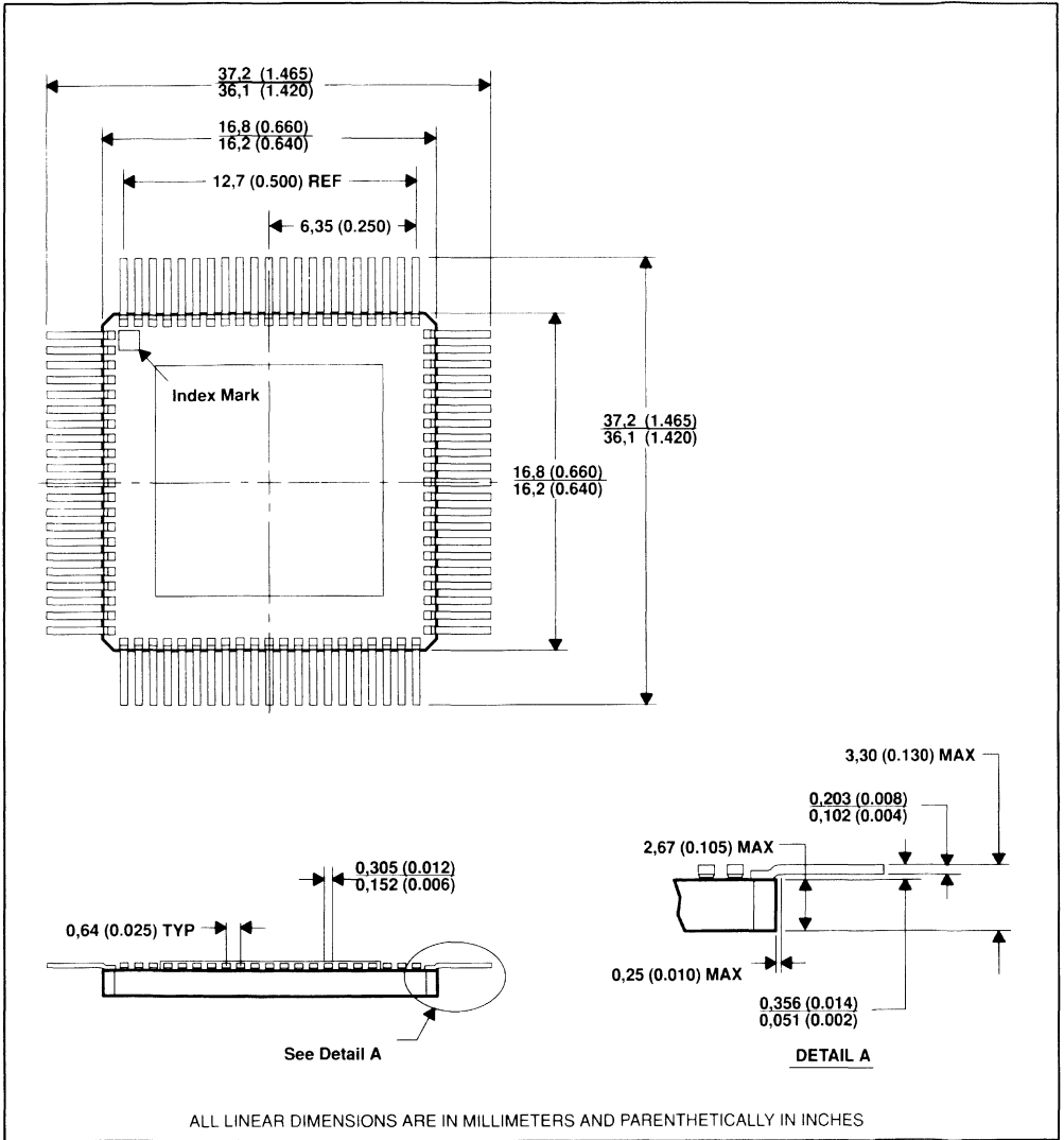
Figure 49. 84-Pin Ceramic Quad Flat Package
