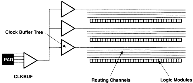
Figure 1–4. Dedicated Clock Buffer Network
