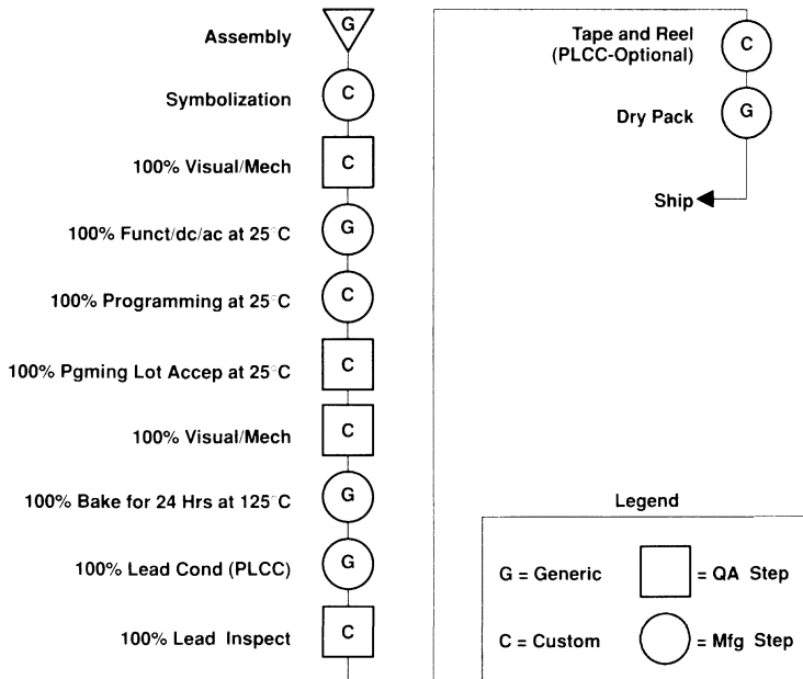
Figure 7. TI P-FPGA Factory Process Flow
