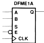
Figure 26. Multiplexed-Input Flip-Flops
