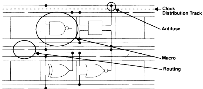
Figure 1-2. Architecture Detail
