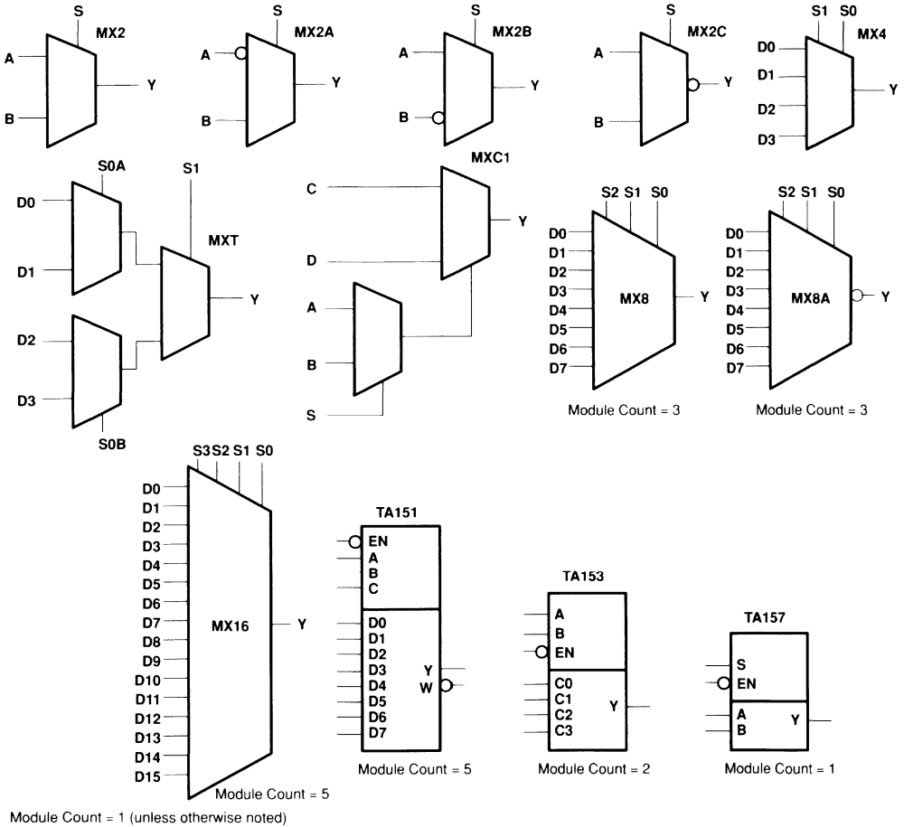
Figure 20. Multiplexers
