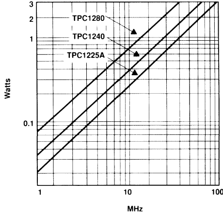
Figure 6. TPC12 Series Power Estimates
