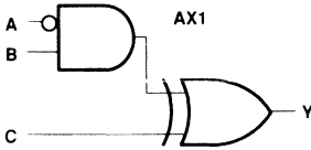
Figure 11. XOR/XNOR Gates
