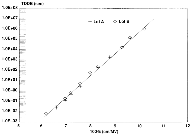
Figure 5-4. ONO Reliability (1/E Model)
