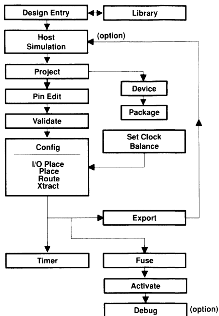
Figure 1. Design Flow
