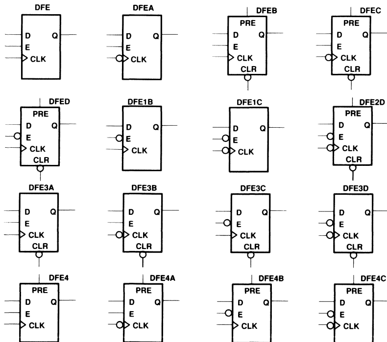
Figure 24. D-Type Flip-Flops With Enable
