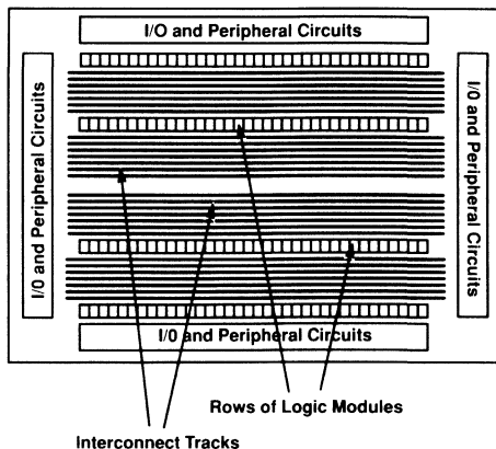
TPC10 Series FPGA Die Architecture
