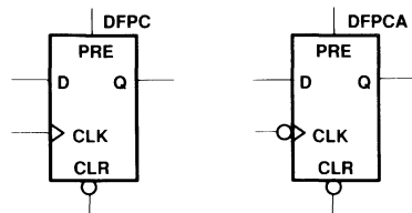
Figure 23. D-Type Flip-Flops
