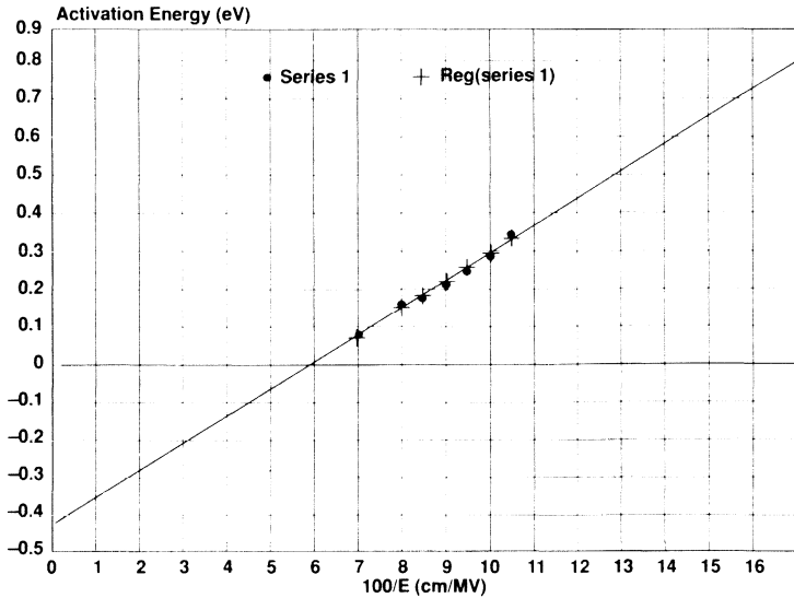
Figure 5–7. Activation Energy versus 1/IE
