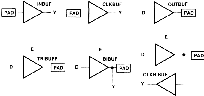
Figure 19. I/O Buffers
