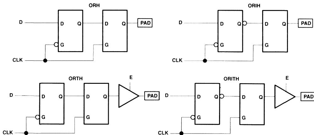
Figure 23. Output Buffers With Registers
