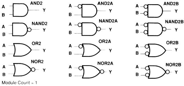
Figure 7. 2-Input Gates
