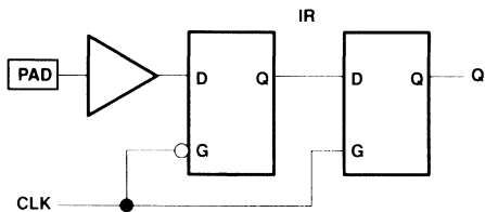
Figure 21. Input Buffer With Register
