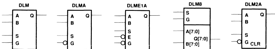
Figure 22. D-Types Latches (Continued)
