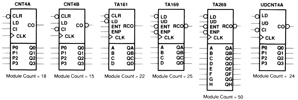
Figure 30. Counters
