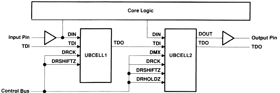
Figure 7. Boundary Register Using UBCELL1
