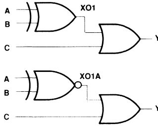
Figure 12. XOR-OR/XNOR-OR Gates
