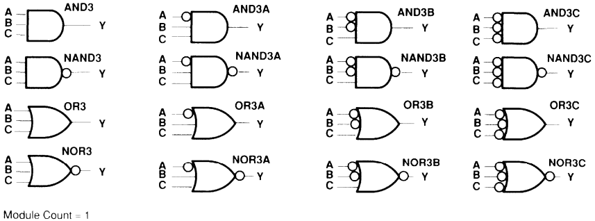
Figure 8. 3-Input Gates
