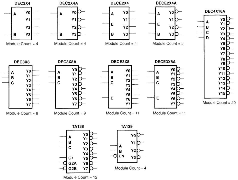
Figure 31. Decoders
