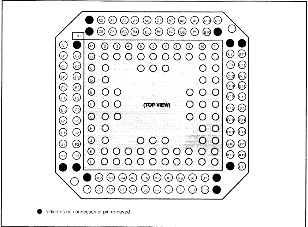
Figure 46. 84-Pin PGA Actionprobe
