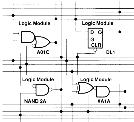
Figure 2. Partial View of TPC10 Series Interconnection Capability
