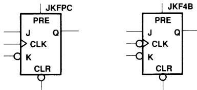
Figure 25. J-K̄ Flip-Flops
