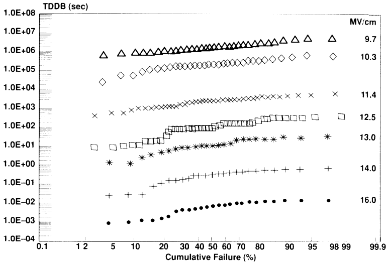
Figure 5-3. TDDB Distribution
