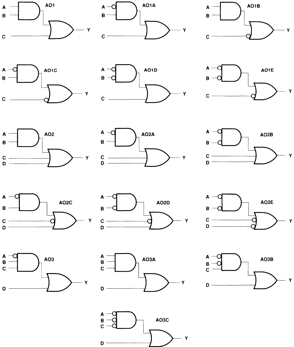
Figure 15. AND-OR/AND-NOR Gates
