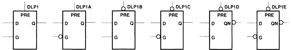
Figure 27. D-Type Latches
