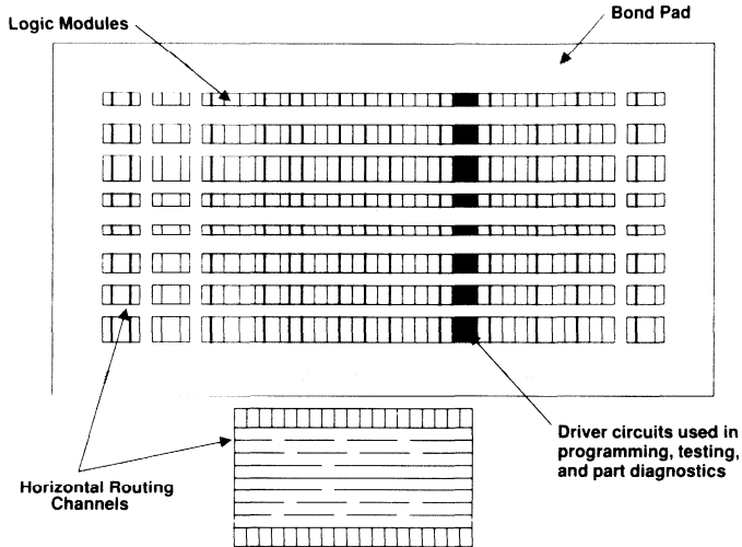
Figure 1-2. Architecture Detail
