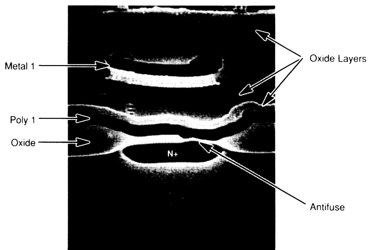
Figure 5–1. Antifuse SEM Cross-Section
