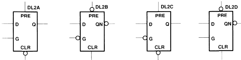
Figure 22. D-Type Latches
