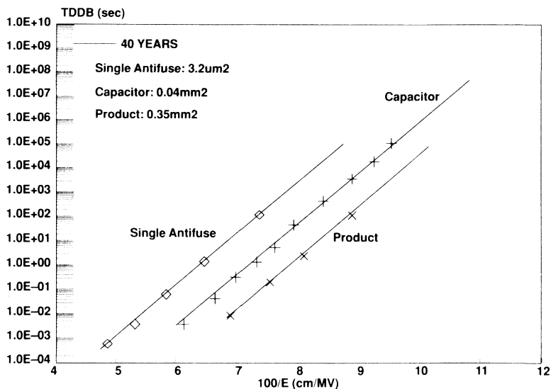
Figure 5–2. Field Accelerated Test
