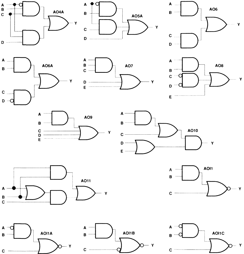
Figure 14. AND-OR/AND-NOR Gates (Continued)
