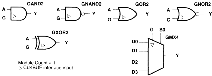
Figure 33. Clock Buffer (CLKBUF) Interface
