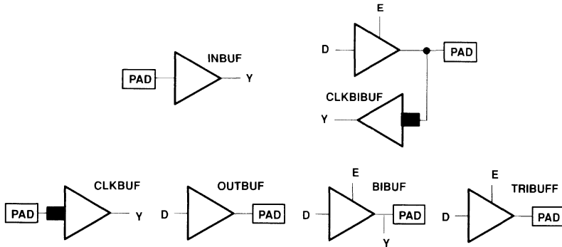
Figure 17. Buffers
