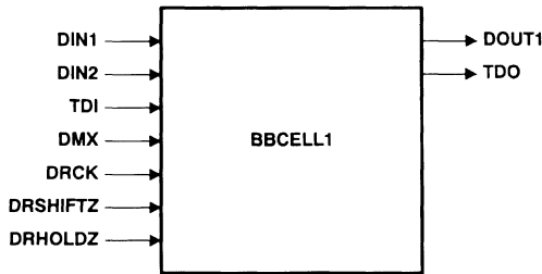
Figure 10. Bidirectional Boundary Cell 1
