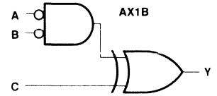
Figure 13. XOR-AND/ XNOR-AND Gates
