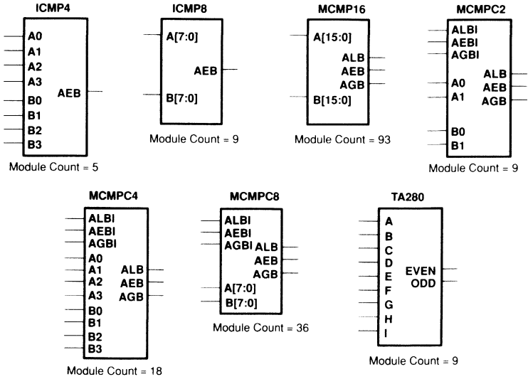
Figure 29. Comparators/Parity Checker
