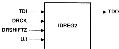
Figure 20. Identification Register 2 Macro
