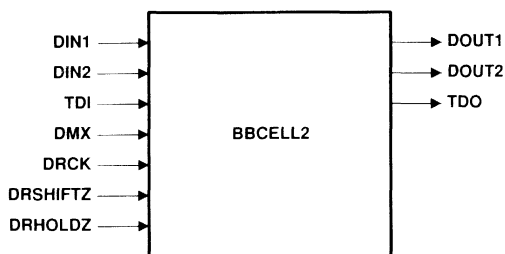
Figure 12. Bidirectional Boundary Cell 2
