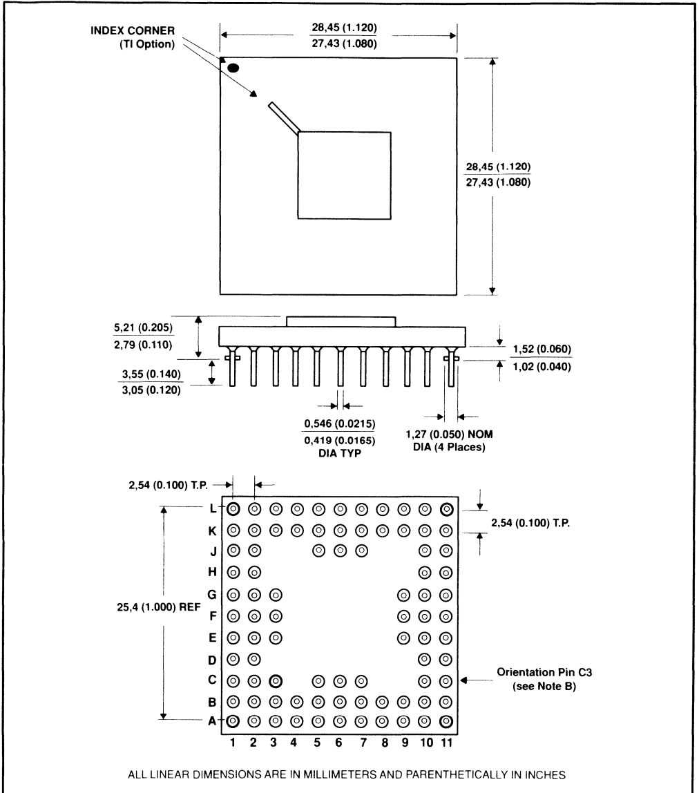
Figure 48. 84-Pin Ceramic Pin-Grid-Array Package
