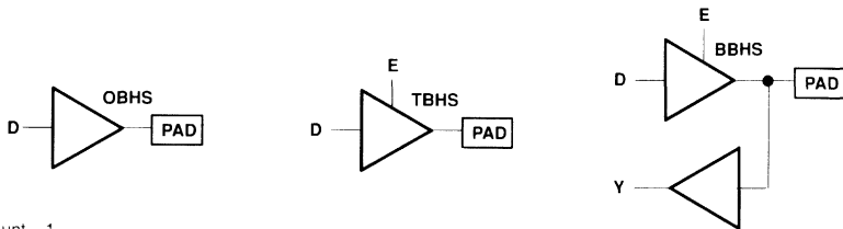
Figure 18. I/O Buffers
