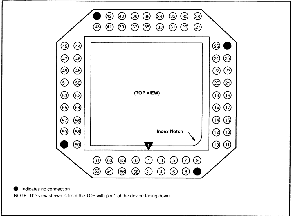
Figure 44. 68-Pin PLCC Actionprobe
