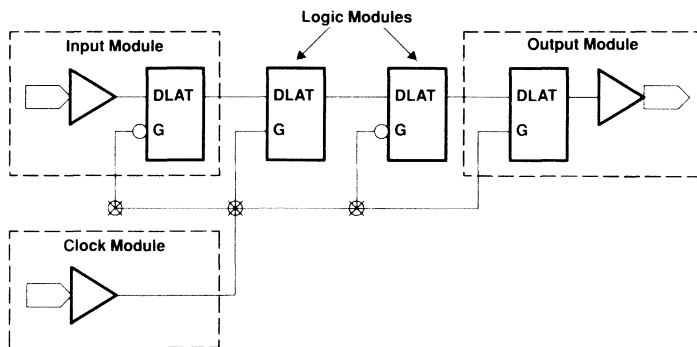
Figure 2. Latched User I/Os
