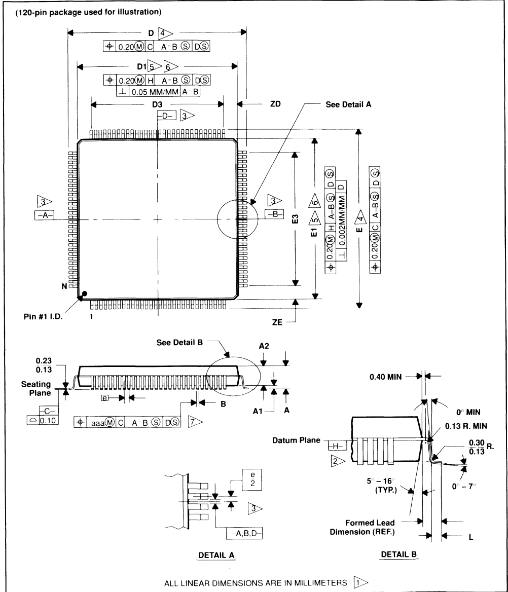
Figure 51. Plastic Quad Flat Packages
