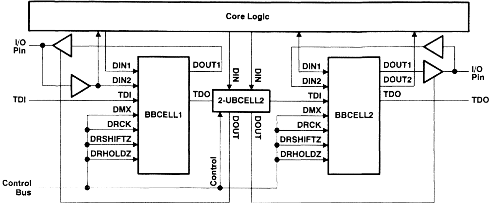
Figure 11. Boundary Register Using BBCELL1
