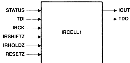
Figure 15. Instruction Register Cell 1
