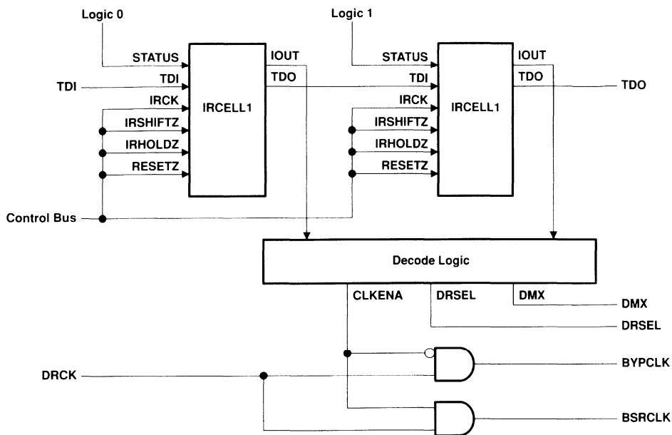
Figure 17. Example Instruction Register
