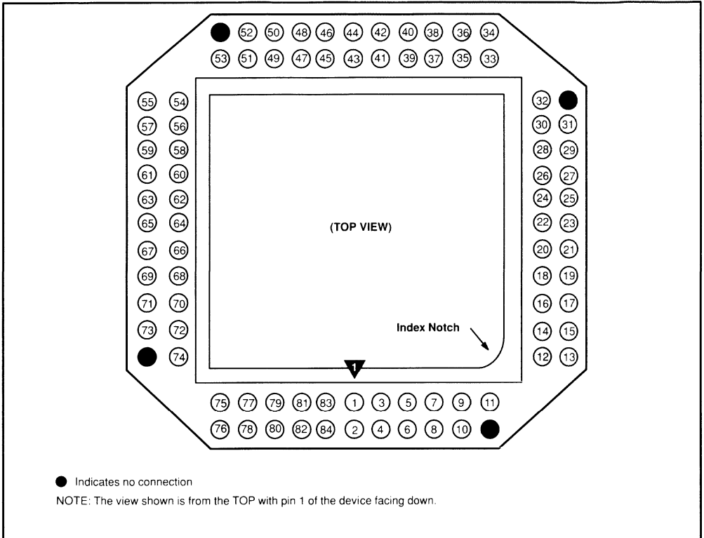
Figure 45. 84-Pin PLCC Actionprobe
