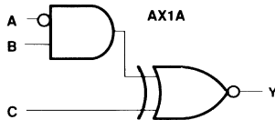
Figure 15. AND-XOR/AND-XNOR Gates
