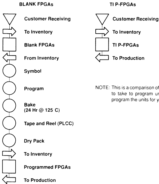
Figure 6. Blank vs TI Programmed FPGA Process Steps
