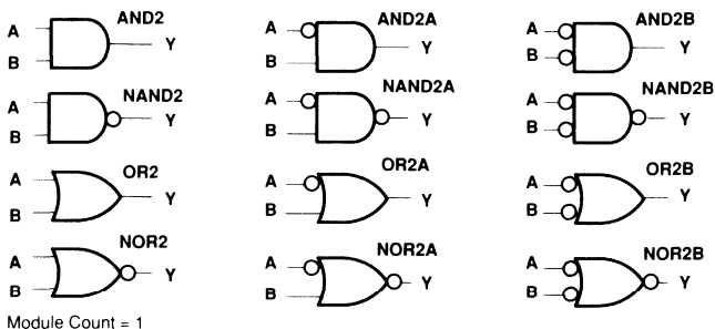
Figure 9. 2-Input Gates
