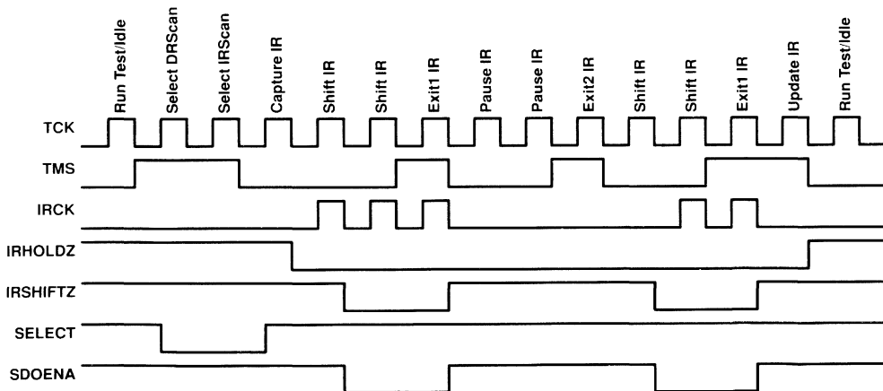
Figure 3. TAP Instruction Register Scan Timing Diagram
