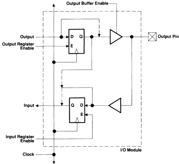
Figure 3. I/O Module With Registered Inputs and Outputs
