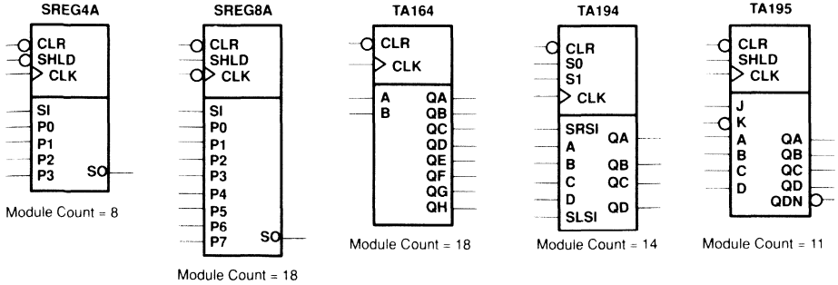
Figure 32. Shift Registers
