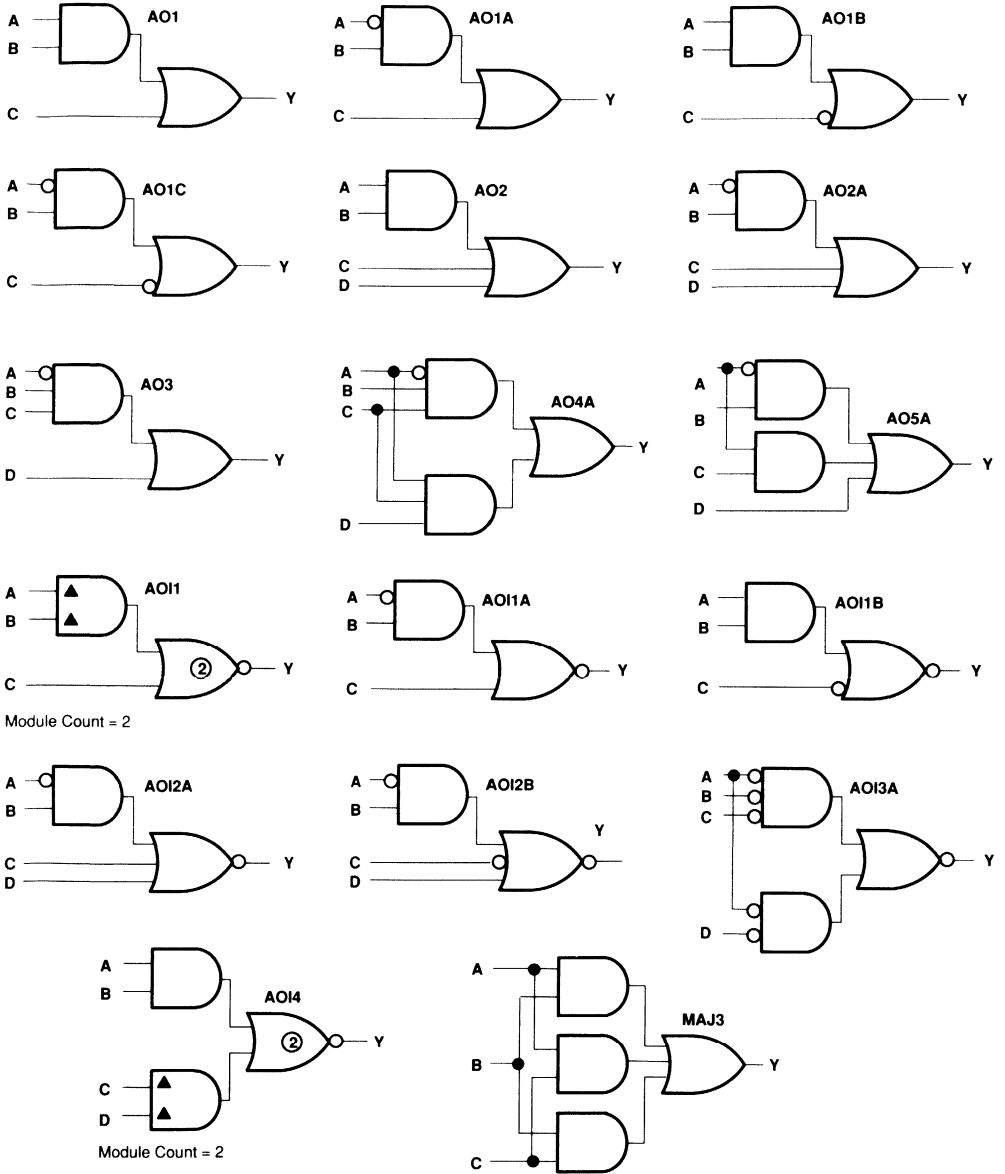
Figure 16. AND-OR/AND-NOR Gates
