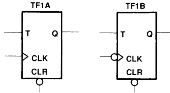
Figure 31. Toggle Flip-Flops
