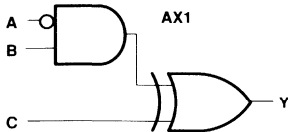
Figure 12. XOR/XNOR Gates
