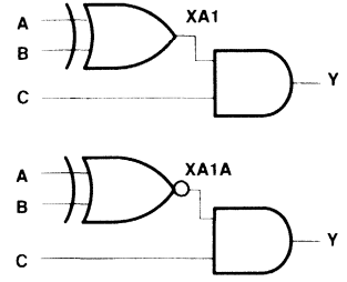
Figure 13. XOR-AND/ XNOR-AND Gates
