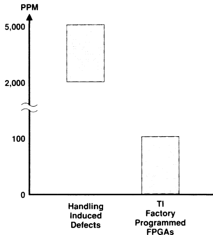
Figure 4. 68-84-Pin PLCC Defect Level Leads
