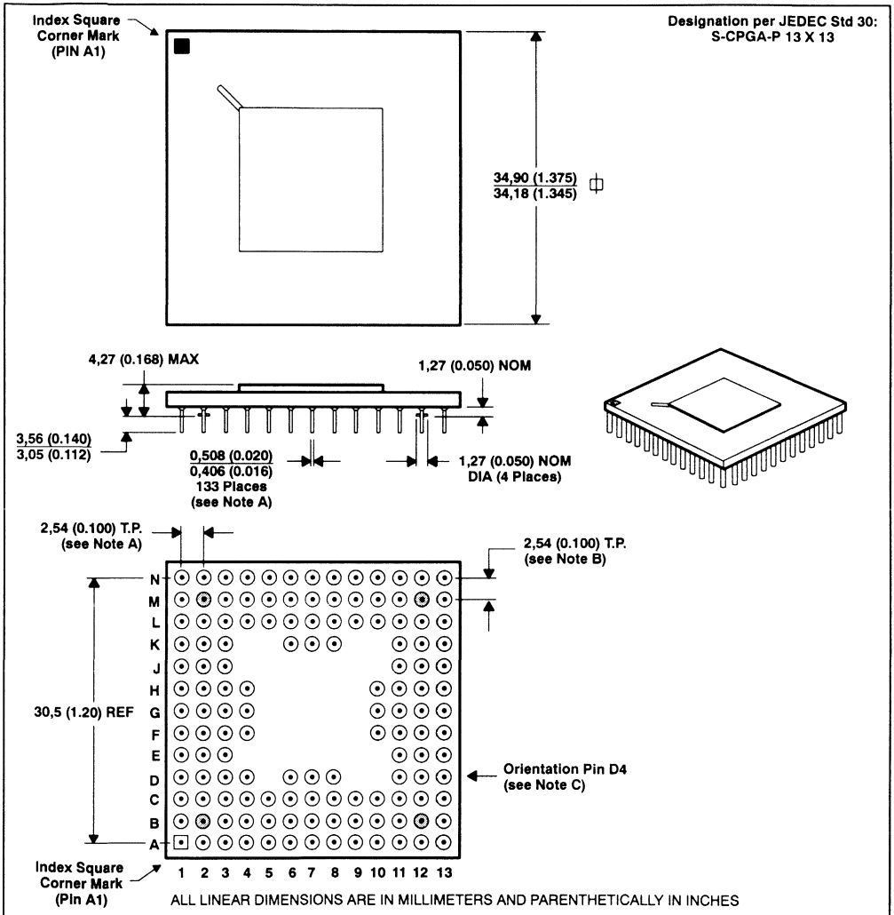
Figure 41. 133-Pin Ceramic Pin-Grid-Array Package
