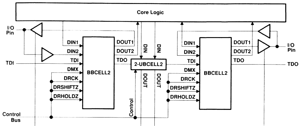
Figure 13. Boundary Register Using BBCELL2
